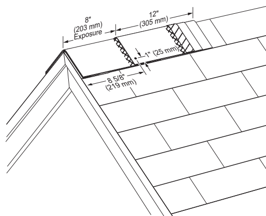
Figure 12-20: Install cap shingles at an 8" exposure and fasten with one nail on each side as shown.
