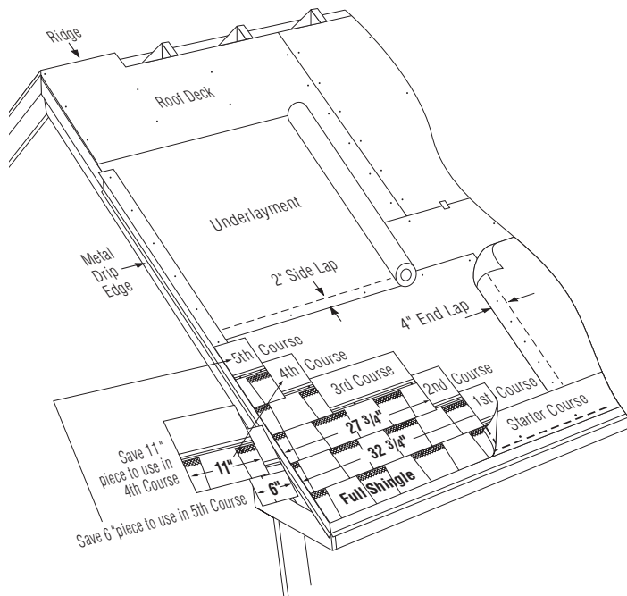
Figure 12-7: Applying the first 5 courses of Landmark.
