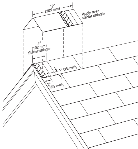
Figure 12-19: Apply a full cap shingle over the starter shingle.
